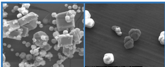
Left: Calcium carbonate crystal formation in the absence of antiscalant
